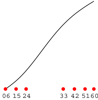
Figure 1: A degree 6 \Delta^1 -invariant diffeomorphism. Note that the control points are ordered.
